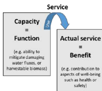
Figure 3 – The capacity concept and its relationship with sustainable provision of ecosystem services
